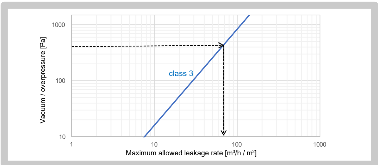
Graph 5 Closed blades leakage class 3 in acc. with EN 1751
