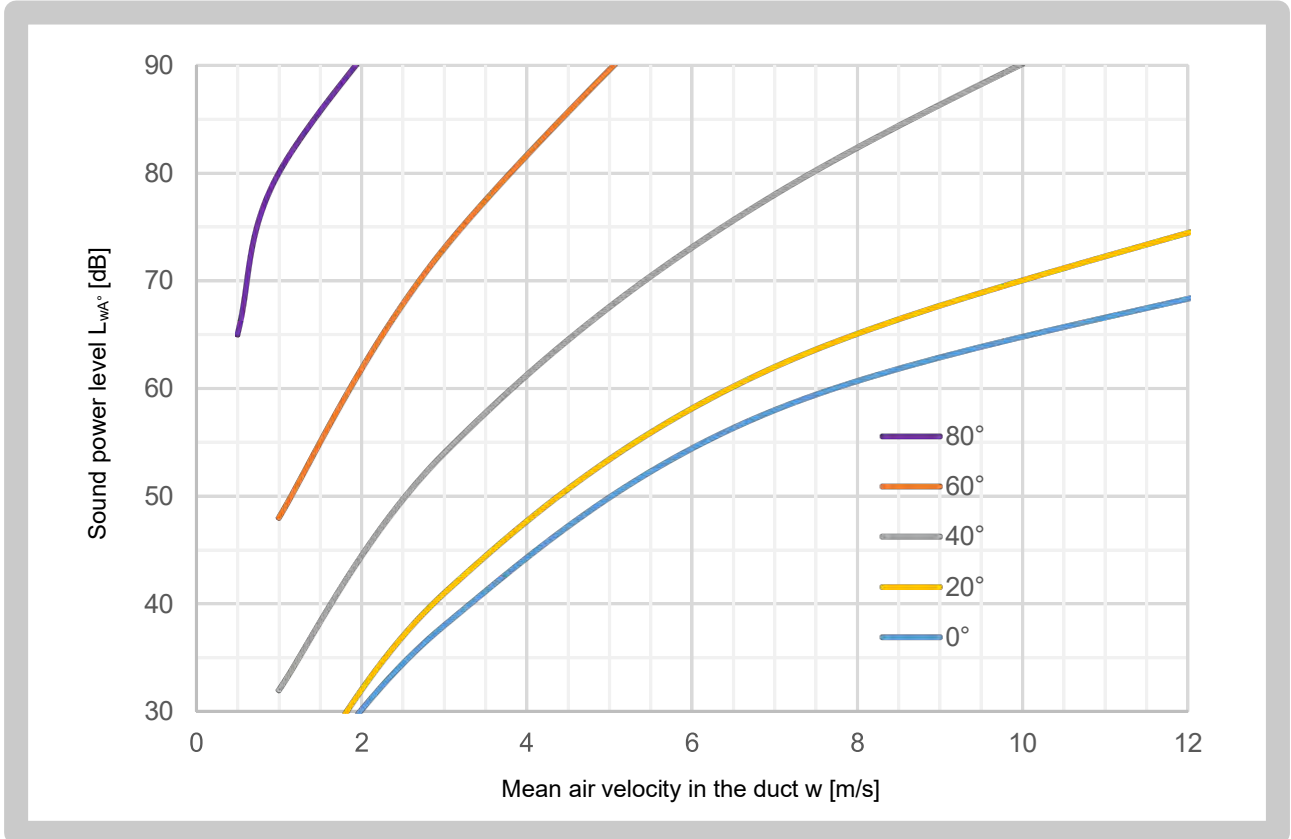
Graph 6 Aerodynamic noise emissions to the duct L_{wA} – sound power level corrected by A-filter for a damper of 1 m 2 cross section
